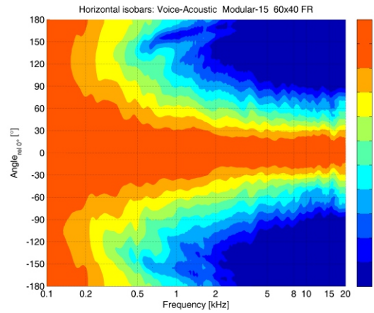
constant directivity over the whole frequency range
